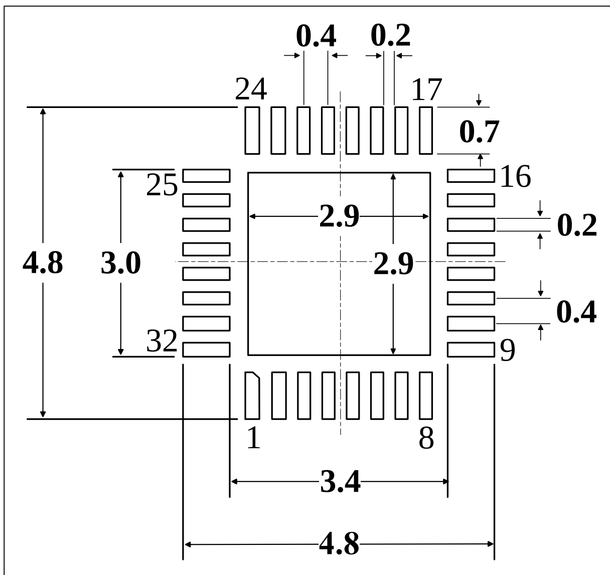
Figure 5-8 QFP32(4mm x 4mm) Recommended footprint (1)
