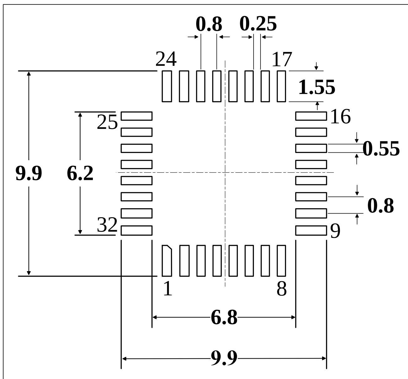
Figure 5-4 LQFP32 Recommended footprint (1)
