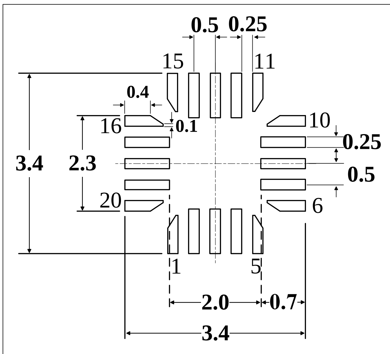
Figure 5-10 UFQFPN20 Recommended footprint (1)
