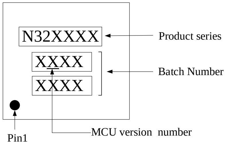
Figure 5-16 UFQFPN20 screen printing instructions
