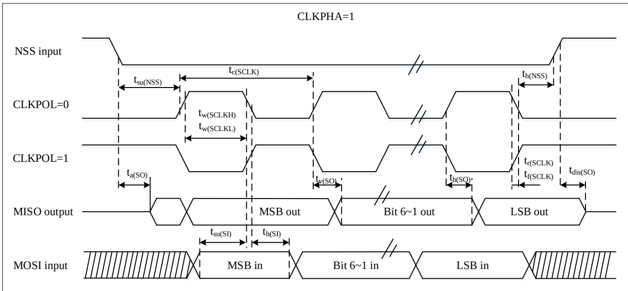
Figure 4-13 SPI sequence diagram - slave mode and CPHA=1 (1)
