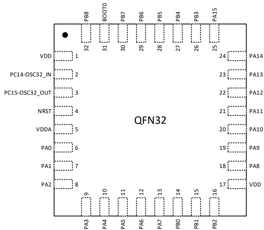
Figure 3-4 N32G031 Series QFN32 (4mmx4mm) pinouts
