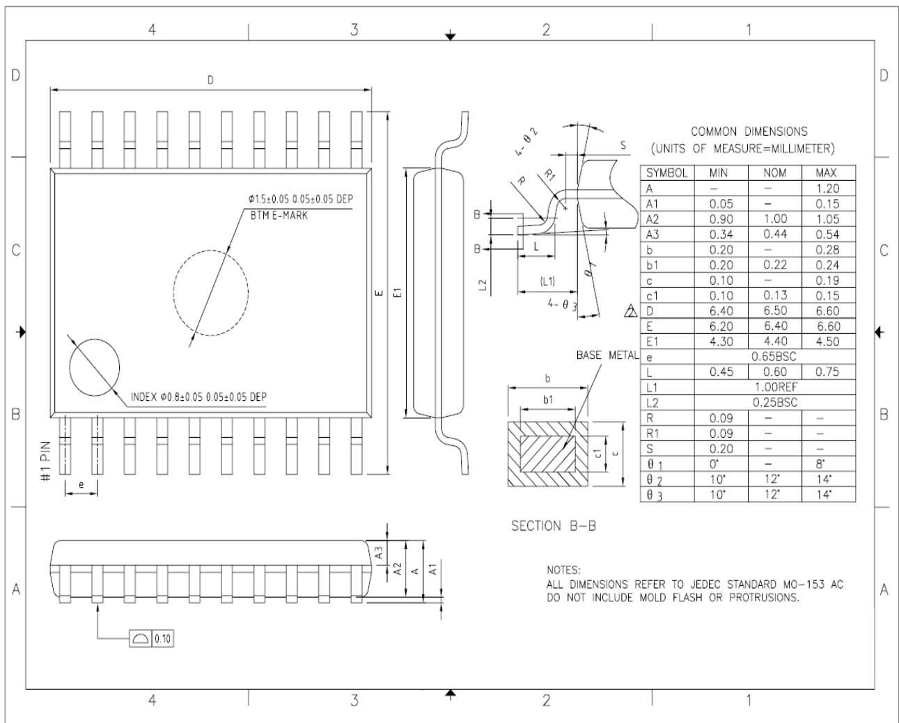
Figure 5-11 TSSOP20 package outline
