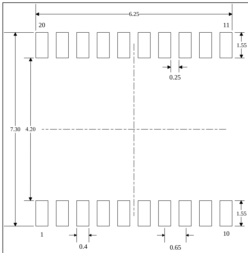
Figure 5-12 TSSOP20 Recommended footprint (1)
