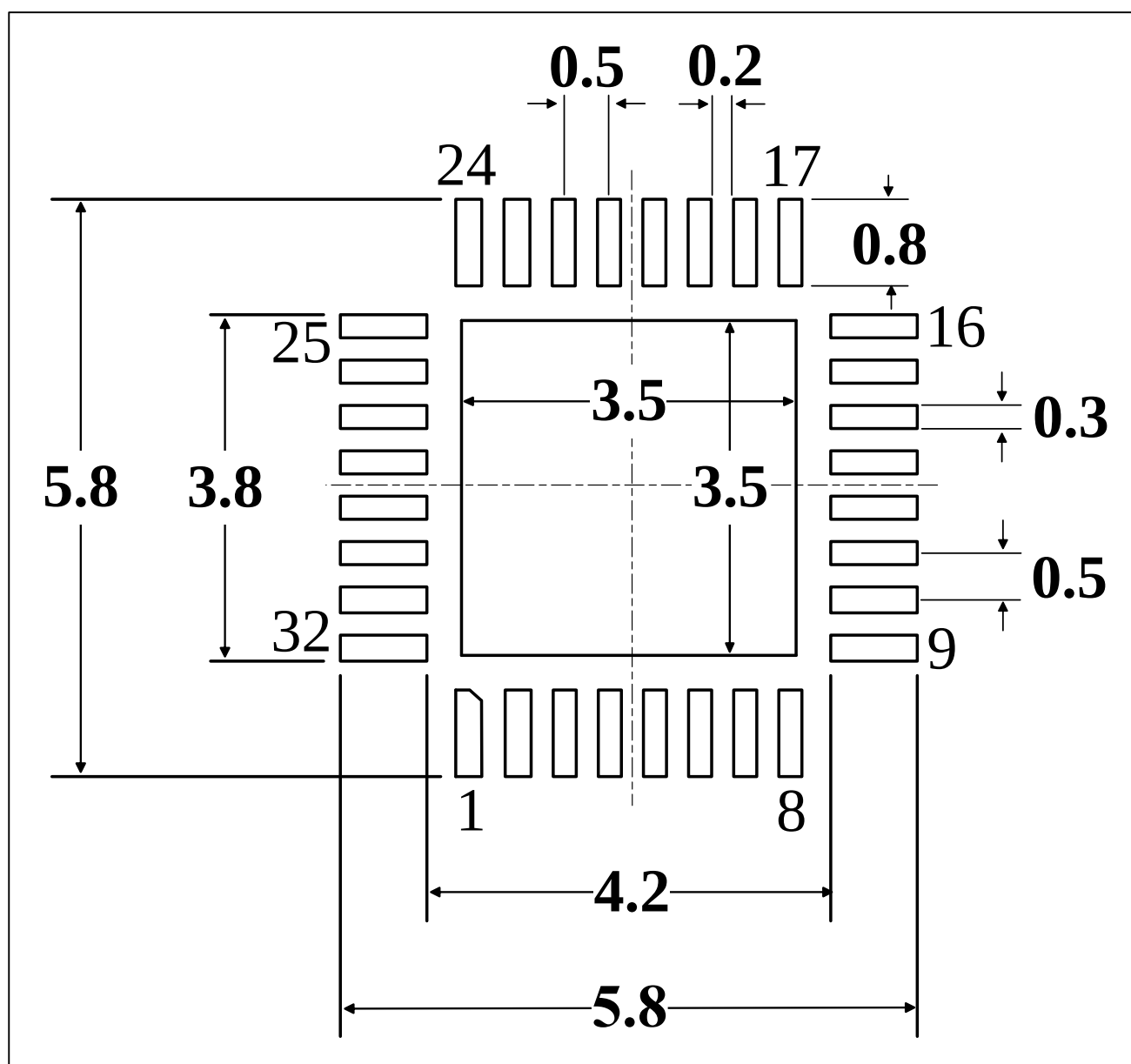
Figure 5-6 QFP32(5mm x 5mm) Recommended footprint (1)
