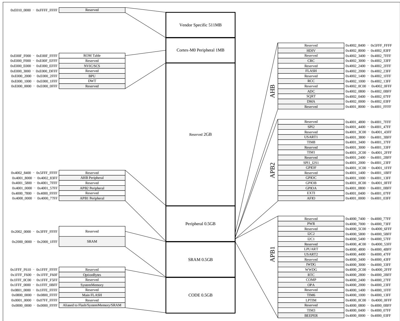
Figure 2-1 Memory address map
