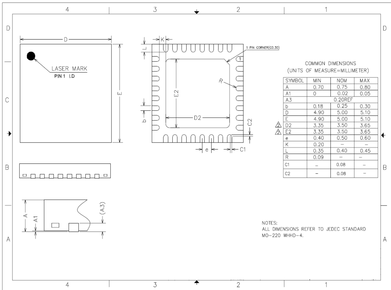
Figure 5-5 QFN32 (5mmx5mm) package outline
