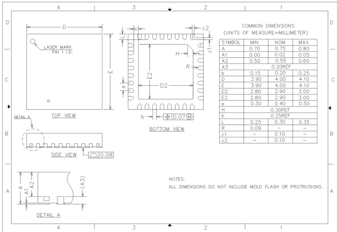
Figure 5-7 QFN32 (4mmx4mm) package outline
