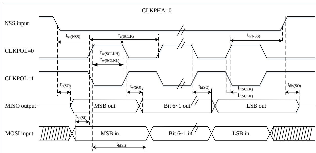
Figure 4-12 SPI sequence diagram - slave mode and CPHA=0
