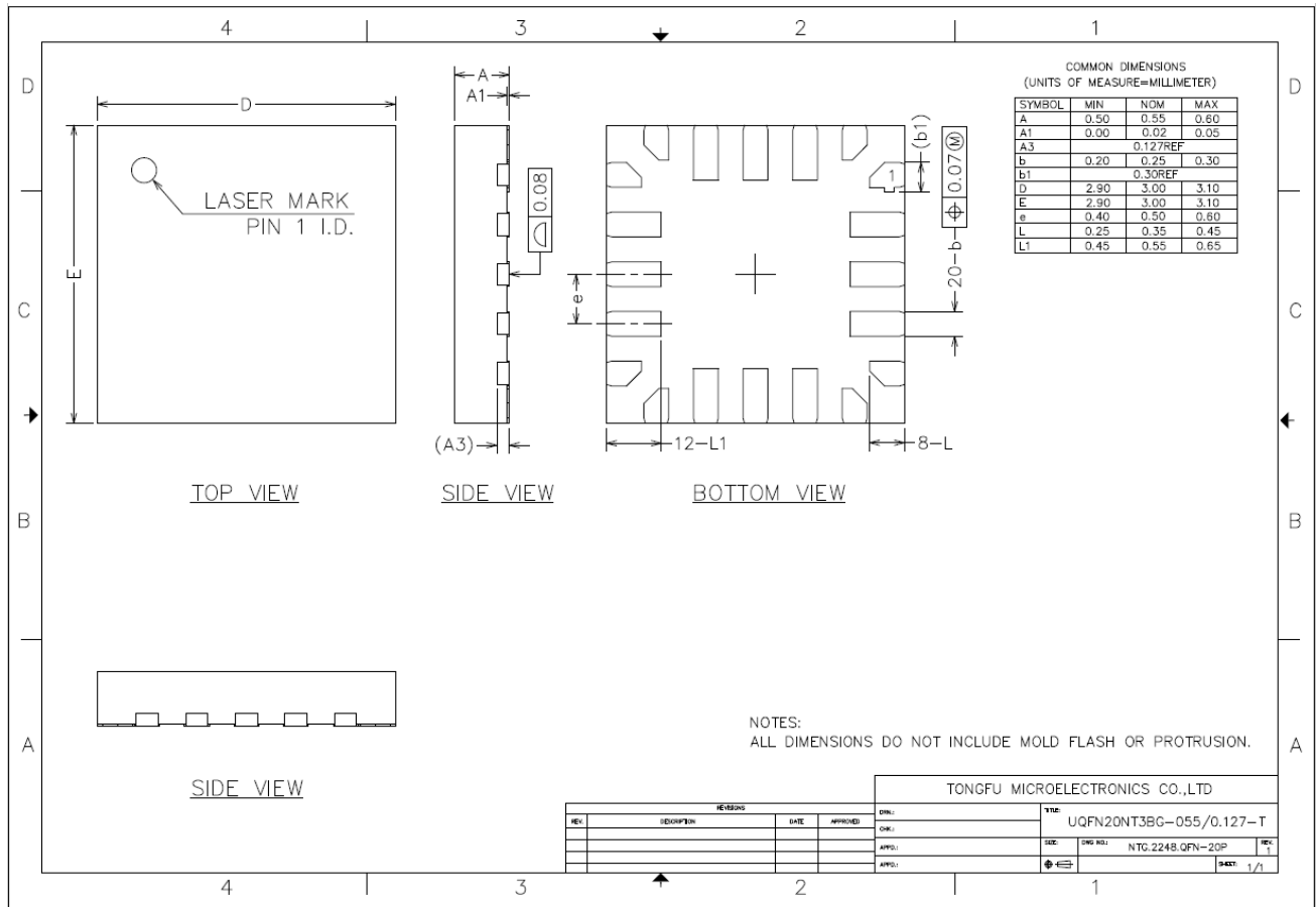
Figure 5-9 UFQFPN20 package outline
