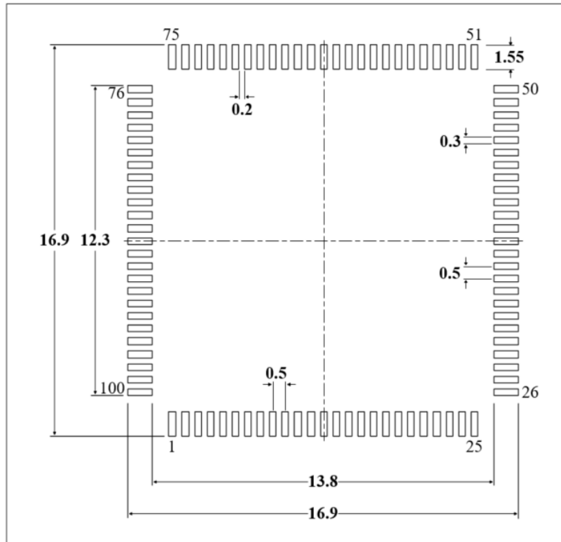
Figure 5-5 Suggestions for LQFP100 Package Pads (1)
