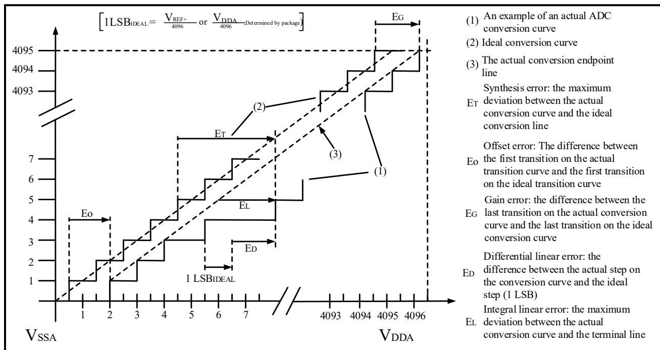
Figure 4-44 ADC Accuracy Characteristics
