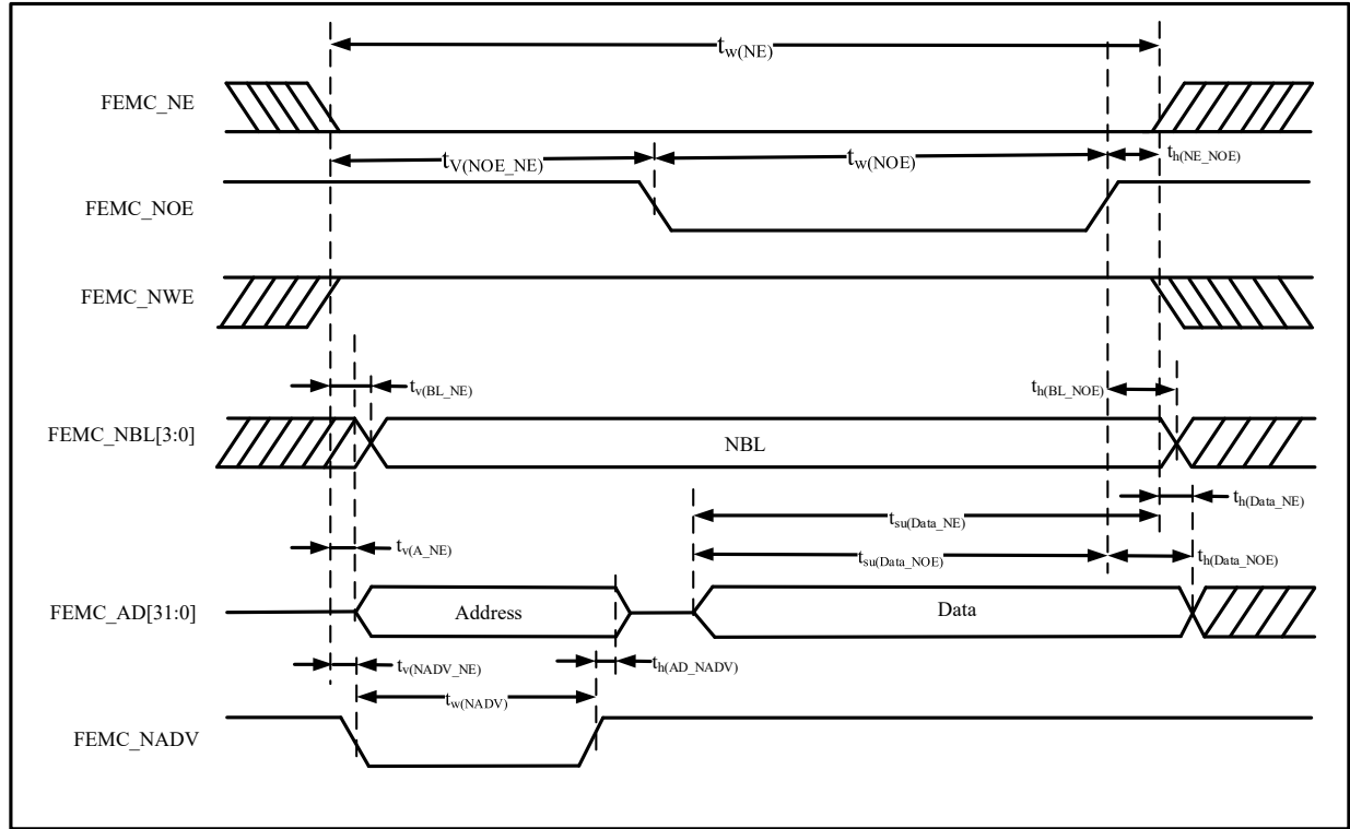
Figure 4-26 Asynchronous Bus Multiplexed PSRAM/NOR Read Operation Waveform
