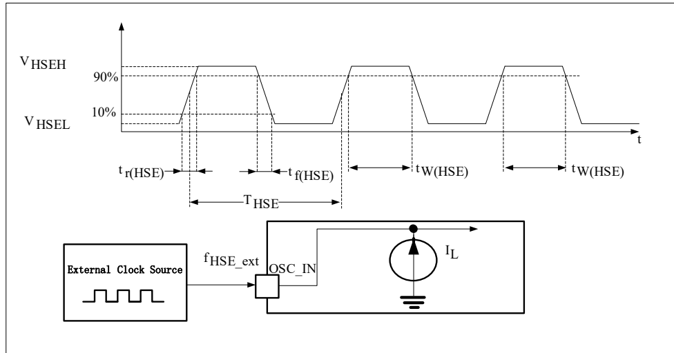
Figure 4-6 High-speed external clock source AC timing diagram
