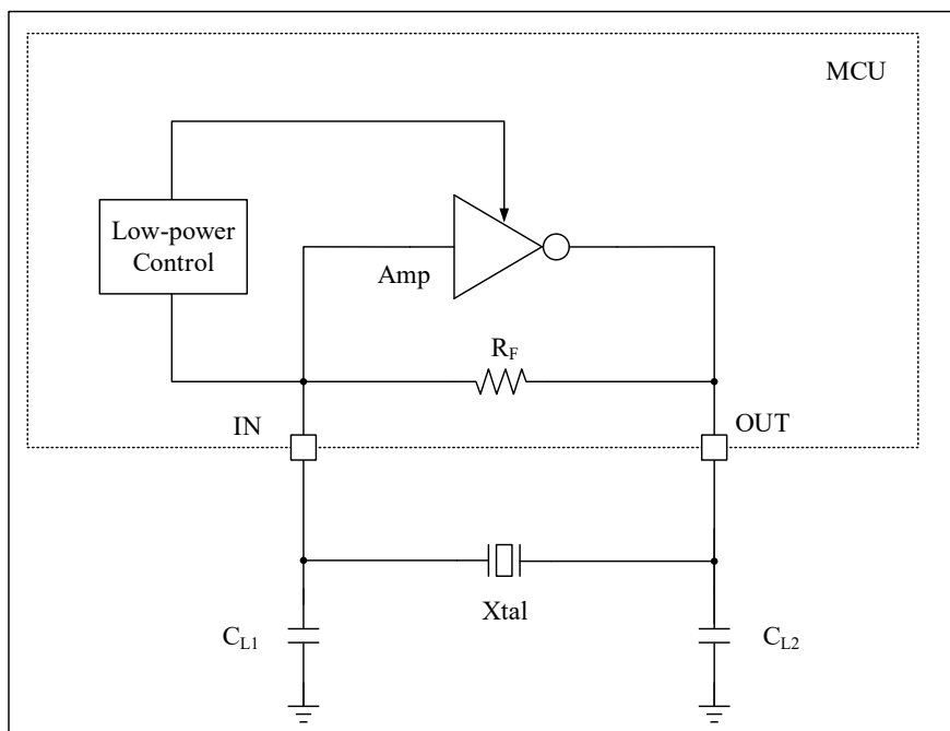
Figure 4-9 Typical Application Using a 32.768kHz Crystal
