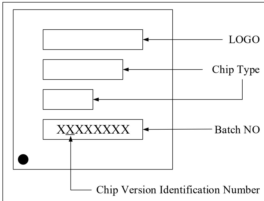
Figure 5-8 Silkscreen Diagram
