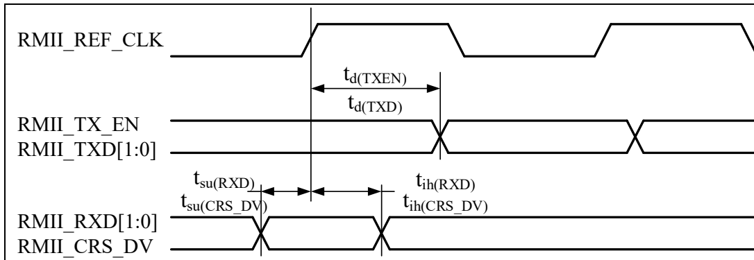
Figure 4-38 RMII Timing Diagram
