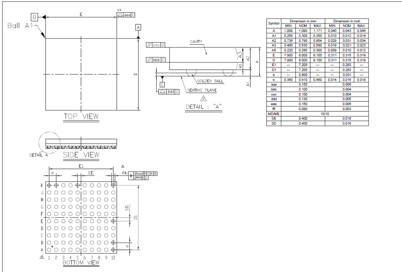
Figure 5-1 BGA100 Package Dimension
