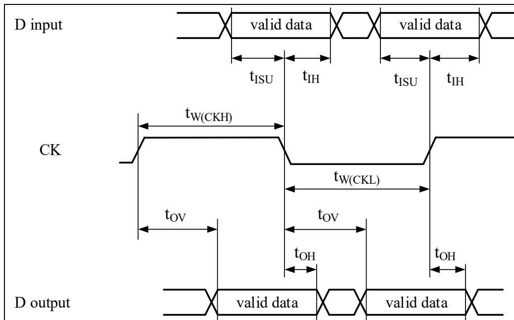
Figure 4-36 SDMMC DDR Mode
