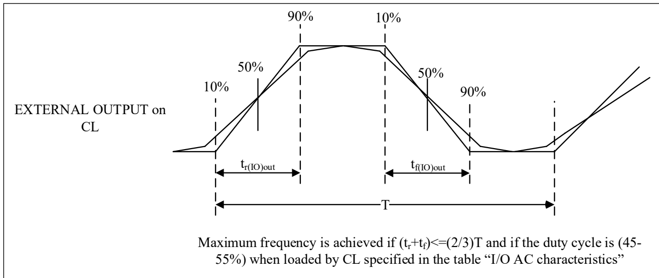
Figure 4-10 Definition of Input/Output AC Characteristics
