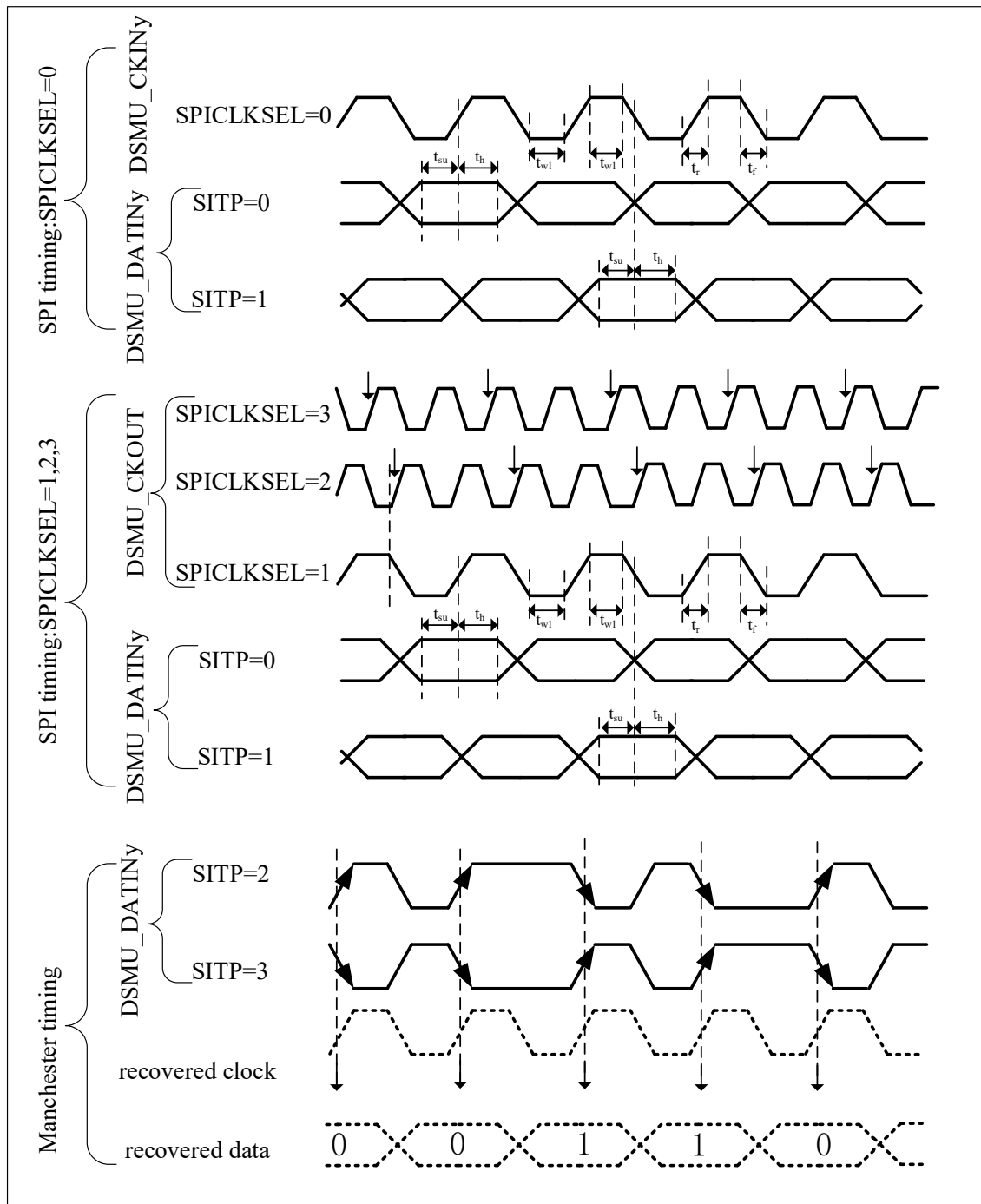
Figure 4-43 DSMU Channel Transceiver Timing Diagram
