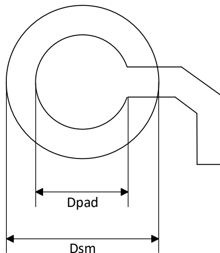
Figure 5-2 Recommended Pads for BGA100 Package
