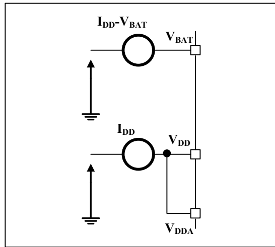
Figure 4-4 Current Consumption Measurement
