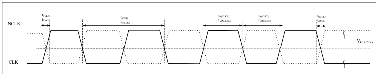
Figure 4-22 xSPI Hyperbus Clock Read Timing Diagram
