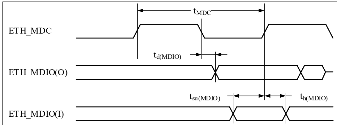
Figure 4-37 MDIO/SMA Timing Diagram
