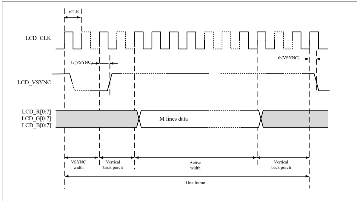
Figure 4-42 LCD-TFT vertical timing diagram
