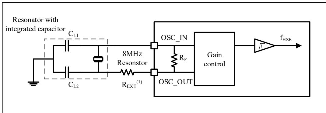
Figure 4-8 Typical application using an 8MHz crystal
