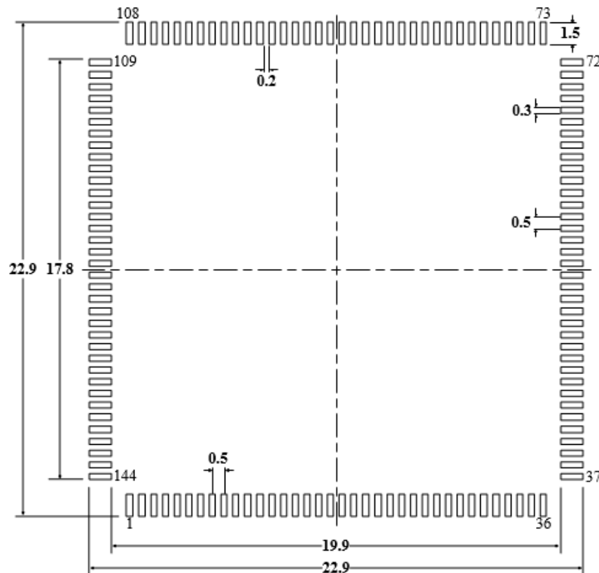
Figure 5-7 Design Recommendations for LQFP144 Package Pads (1)
