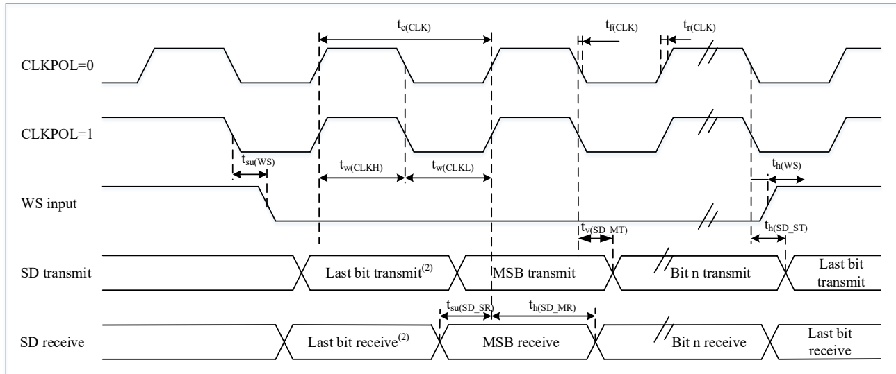
Figure 4-18 I2S Master Mode Timing Diagram (Philips Protocol) (1)
