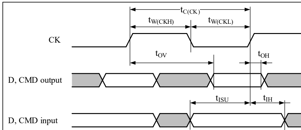
Figure 4-35 SDMMC DDR Mode
