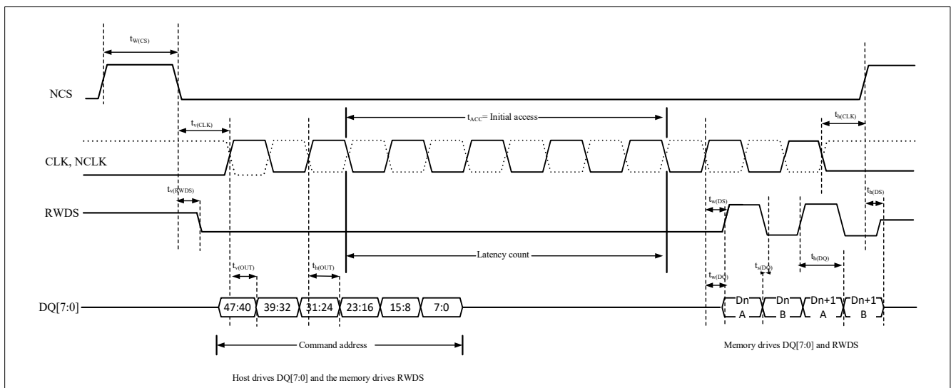
Figure 4-22 xSPI Hyperbus Clock Read Timing Diagram
