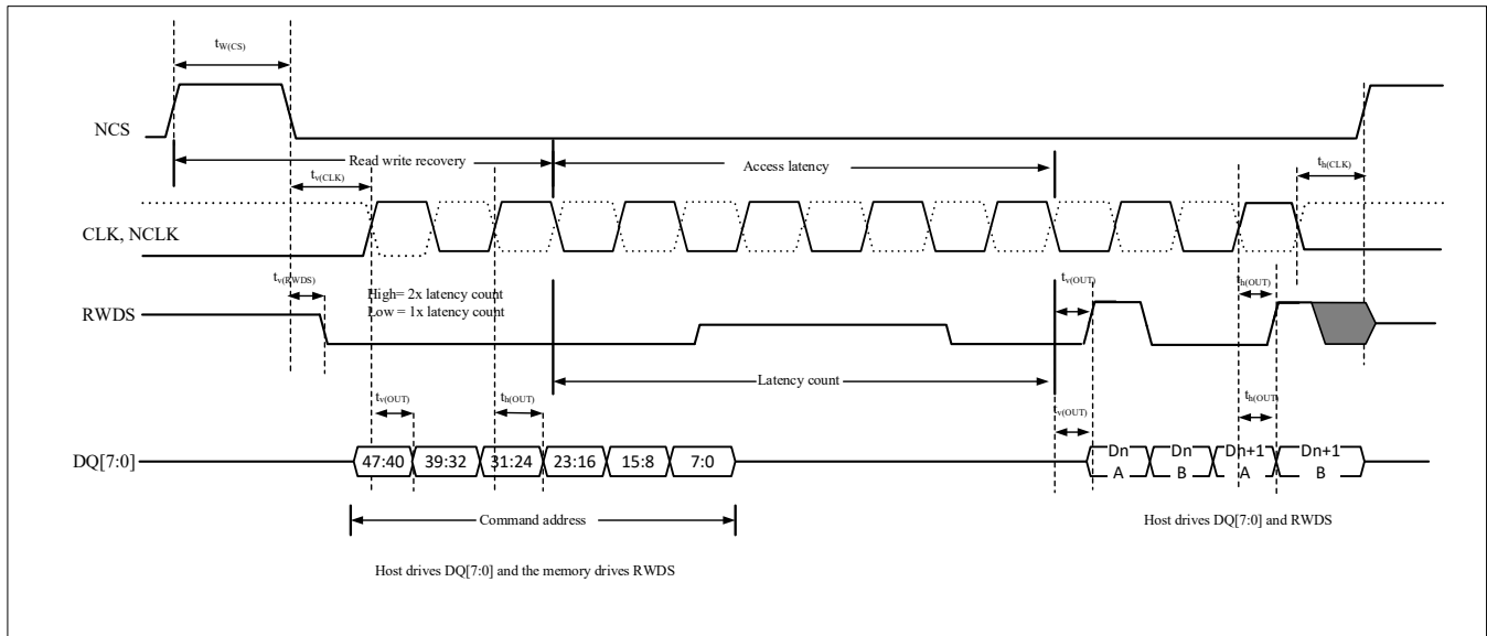
Figure 4-23 xSPI Hyperbus Clock Write Timing Diagram4-1 xSPI Hyperbus
