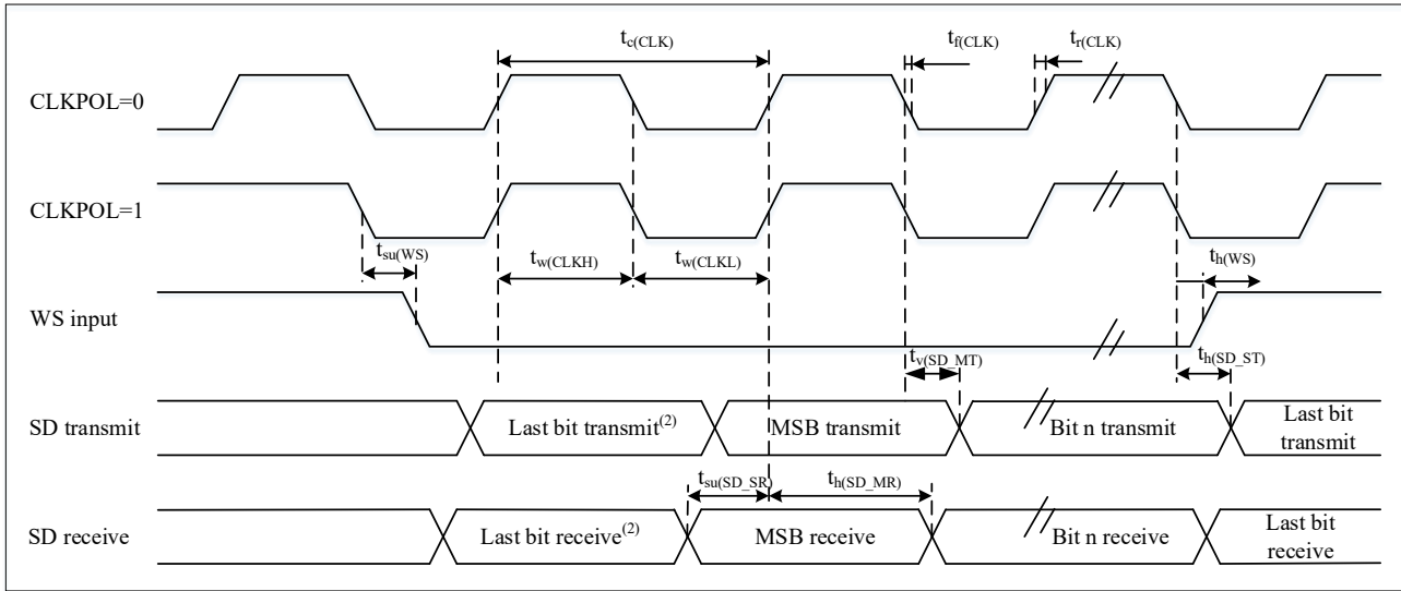
Figure 4-17 I2S Slave Mode Timing Diagram (Philips Protocol) (1)
