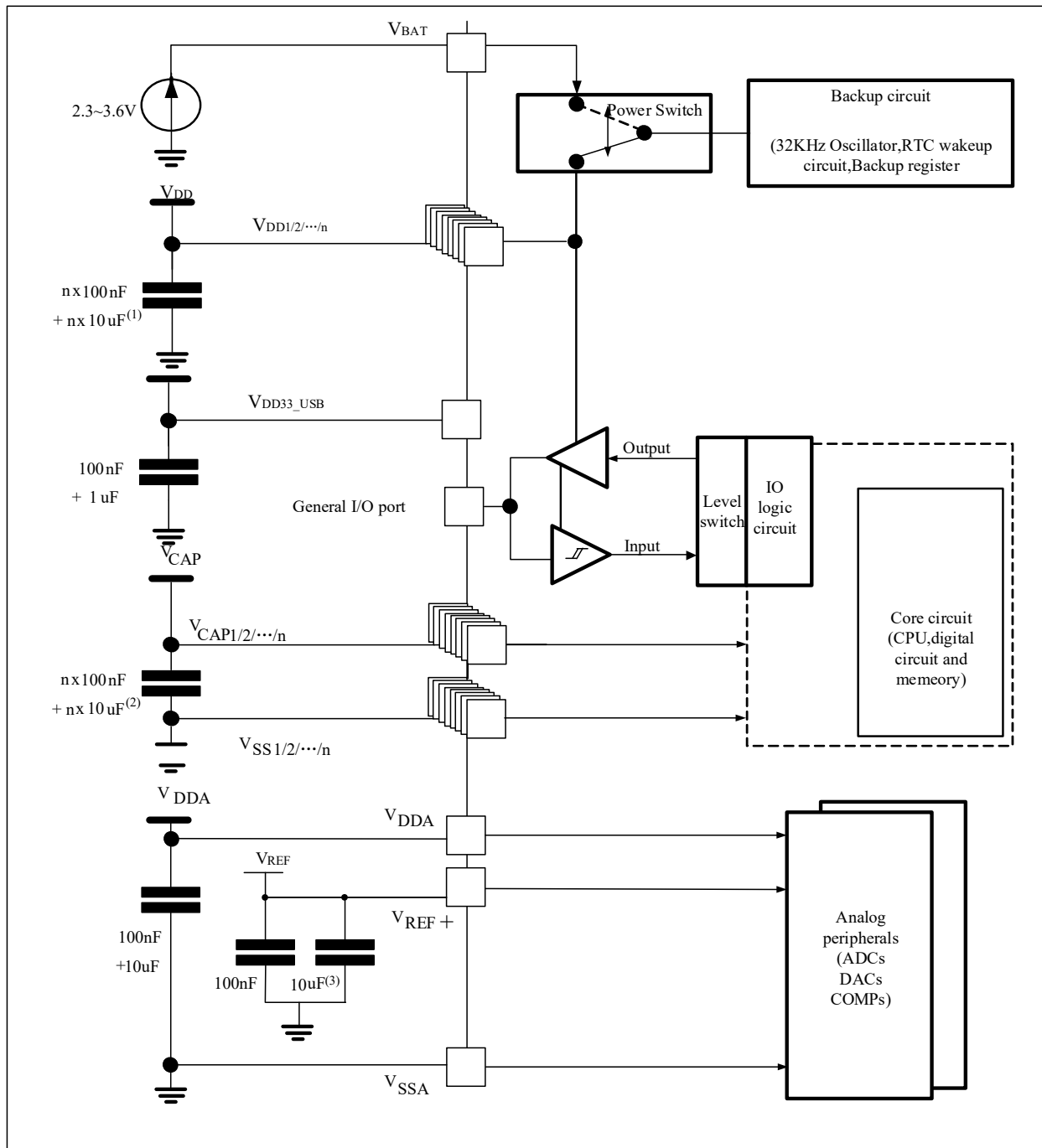
Figure 4-3 Power Supply Scheme
