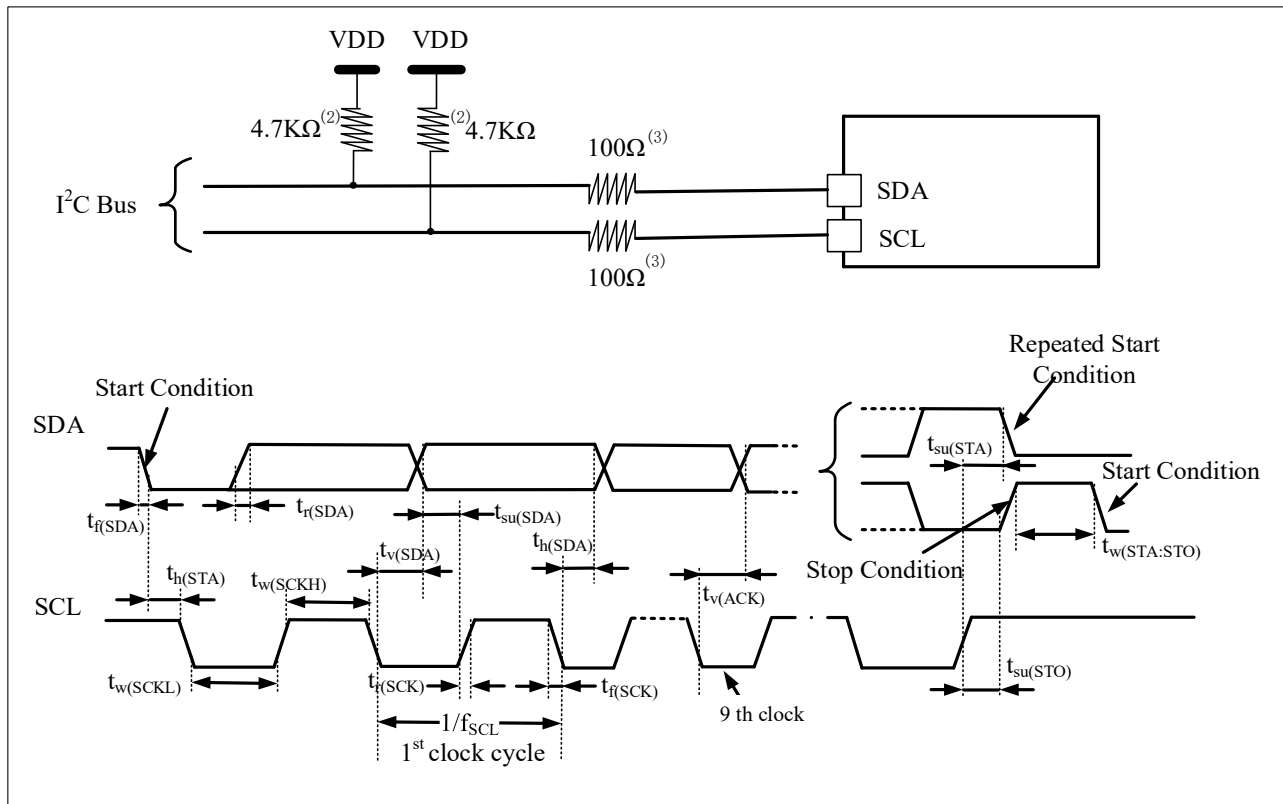
Figure 4-13 I 2 C Bus AC Waveform and Measurement Circuit (1)
