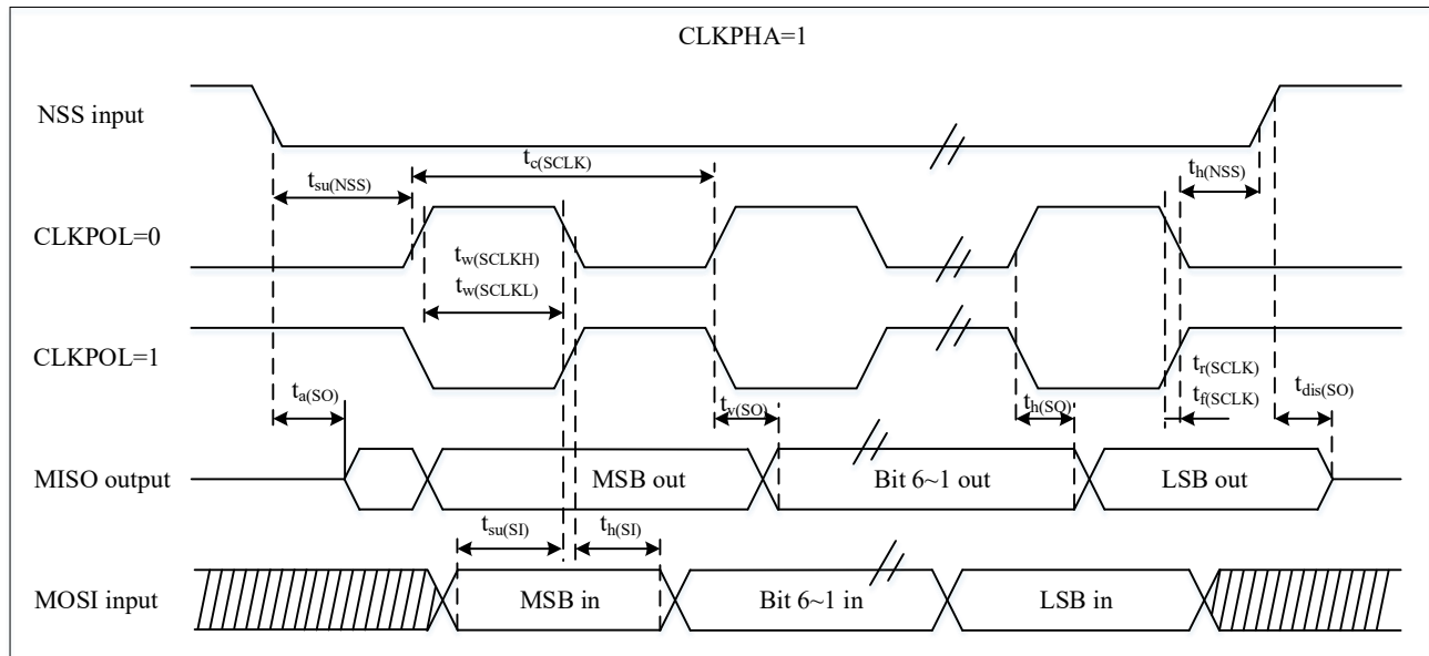
Figure 4-15 SPI Timing Diagram — Slave Mode and CLKPHA=1 (1)
