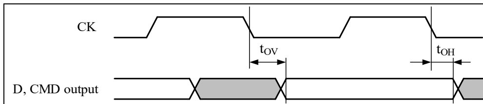
Figure 4-36 SDMMC DDR Mode
