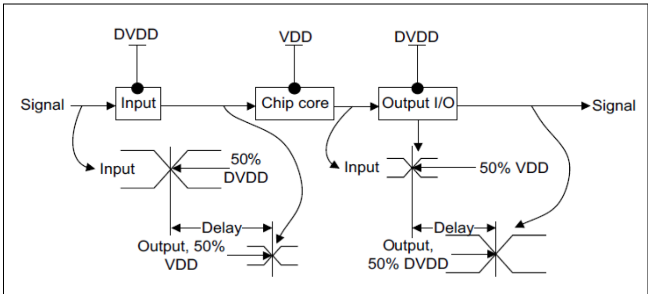
Figure 4-11 Transmission Delay
