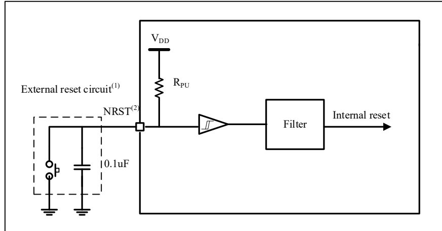
Figure 4-12 Recommended NRST Pin Protection
