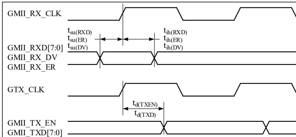
Figure 4-39 MII Timing Diagram
