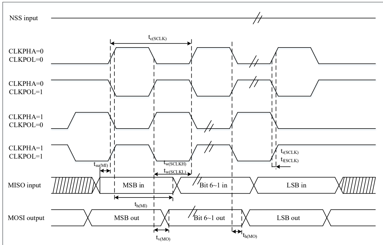
Figure 4-16 SPI Timing Diagram — Master Mode (1)
