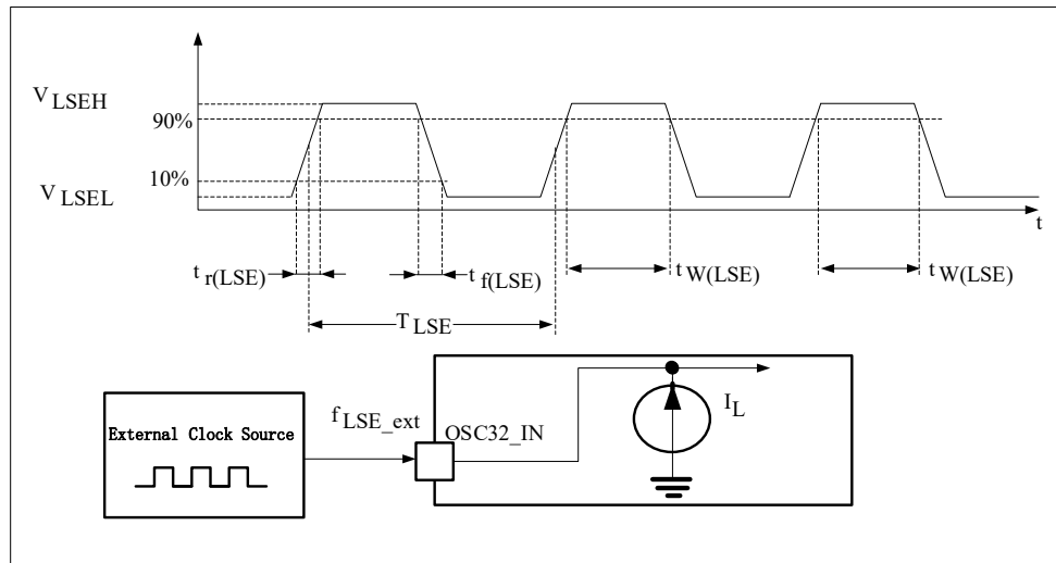
Figure 4-7 Low-speed external clock source AC timing diagram
