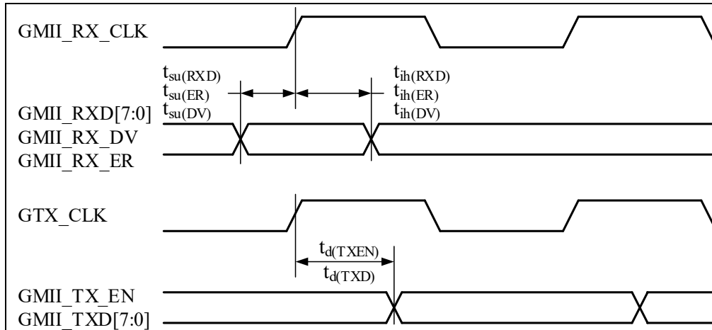
Figure 4-40 MII Timing Diagram
