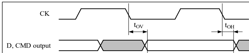
Figure 4-37 SDMMC DDR Mode
