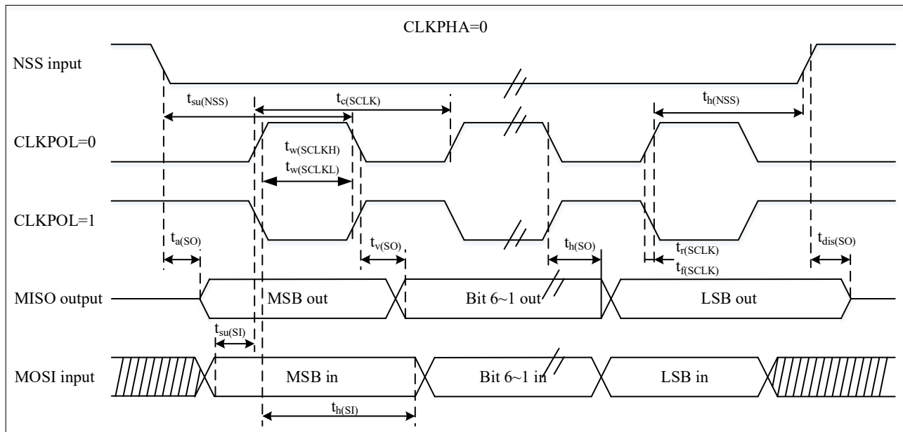
Figure 4-15 SPI Timing Diagram - Slave Mode and CLKPHA=0
