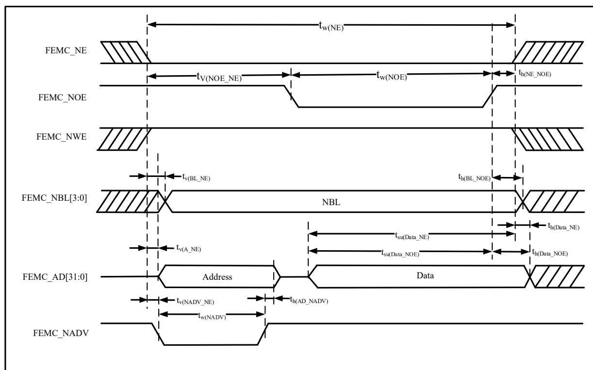
Figure 4-27 Asynchronous Bus Multiplexed PSRAM/NOR Read Operation Waveform
