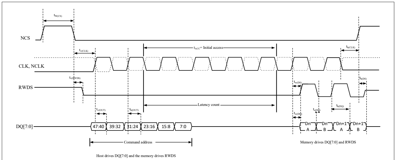
Figure 4-23 xSPI Hyperbus Clock Read Timing Diagram
