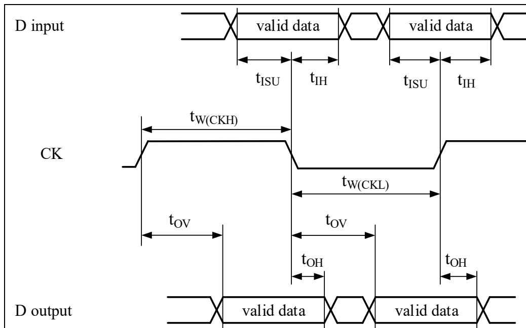
Figure 4-37 SDMMC DDR Mode
