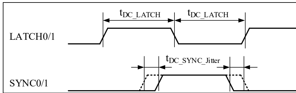
Figure 4-44 ESC Sync/Latch Timing Diagram
