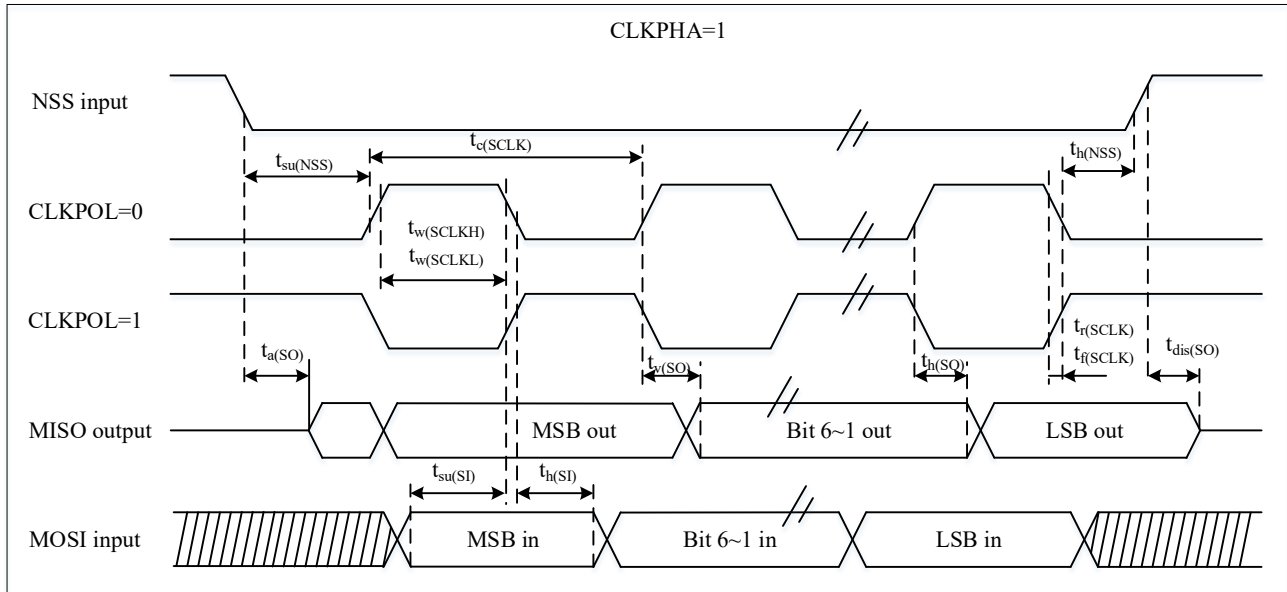
Figure 4-16 SPI Timing Diagram — Slave Mode and CLKPHA=1 (1)
