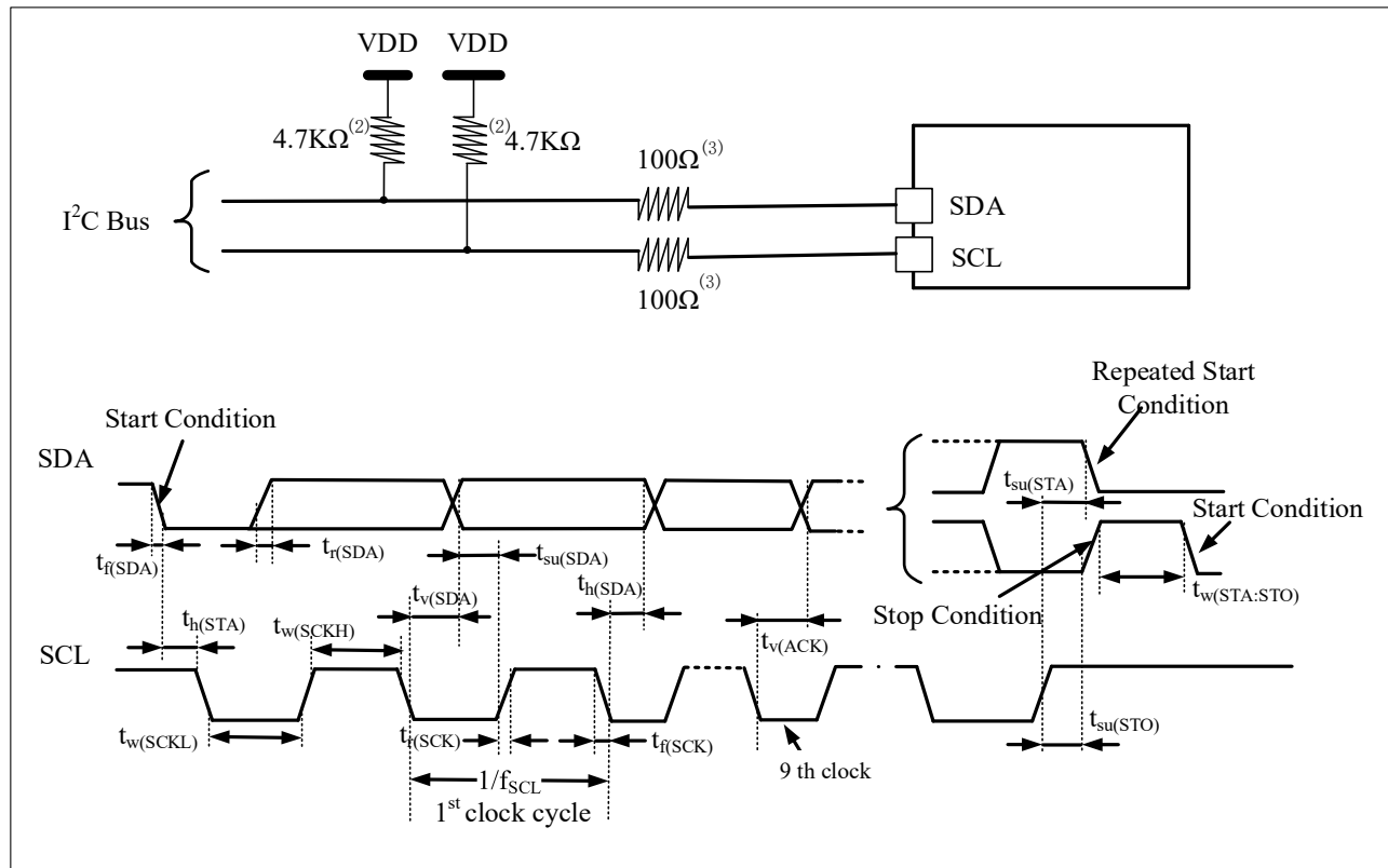
Figure 4-14 I2C Bus AC Waveform and Measurement Circuit (1)
