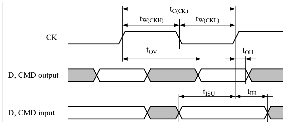
Figure 4-36 SDMMC DDR Mode
