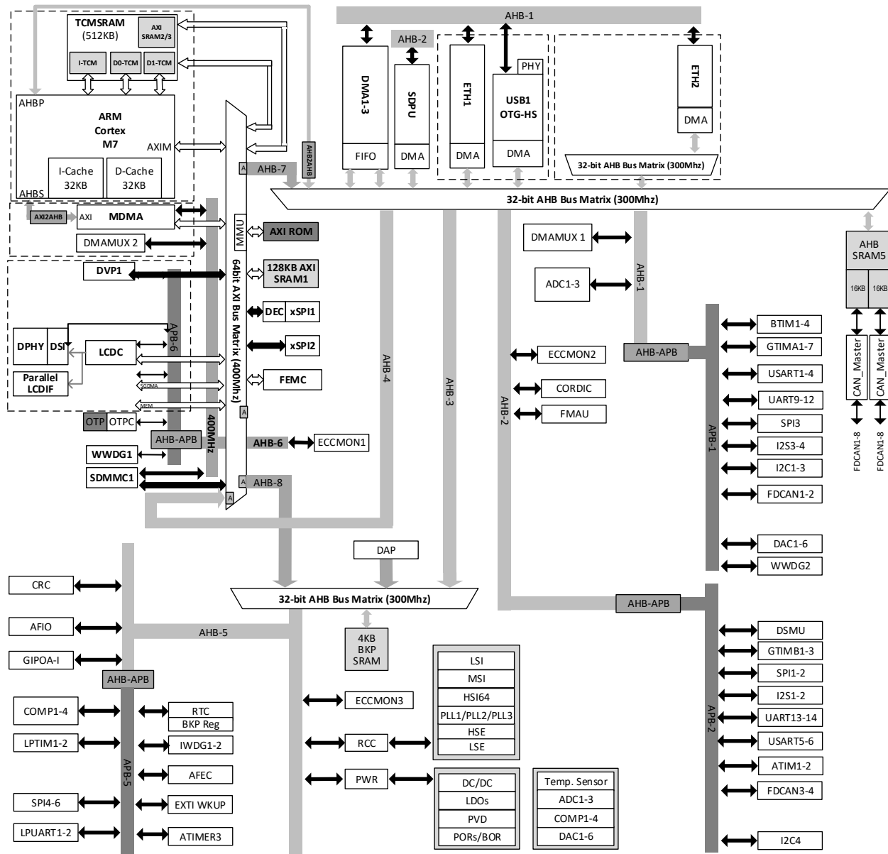
Figure 1-1 N32H735EC System Block Diagram
