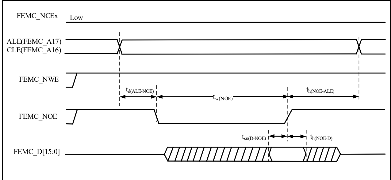
Figure 4-33 NAND Controller Read Operation Waveform
