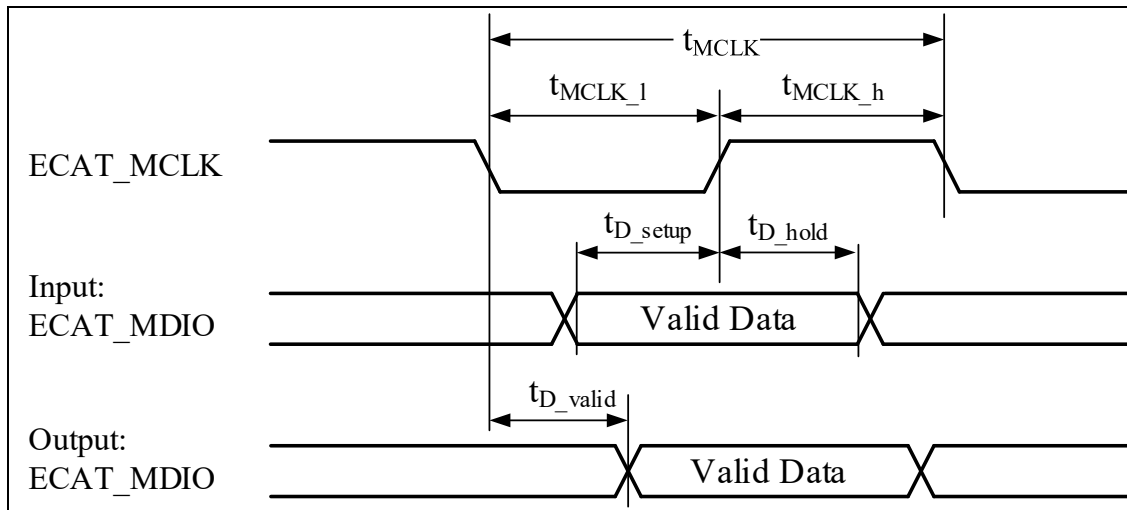
Figure 4-41 MI (MCLK, MDIO) Timing Diagram
