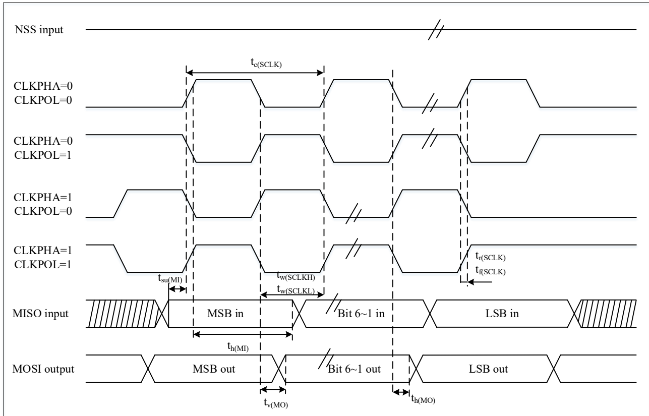
Figure 4-17 SPI Timing Diagram — Master Mode (1)
