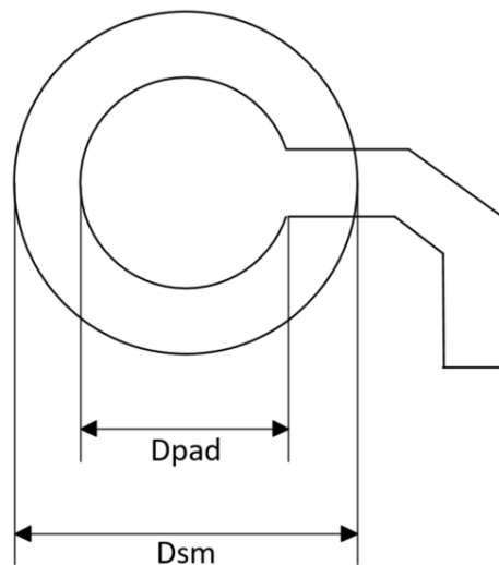
Figure 5-4 Recommended Pads for BGA176+25 Package
