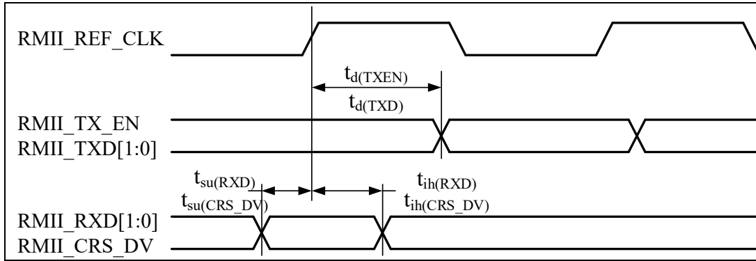
Figure 4-39 RMII Timing Diagram
