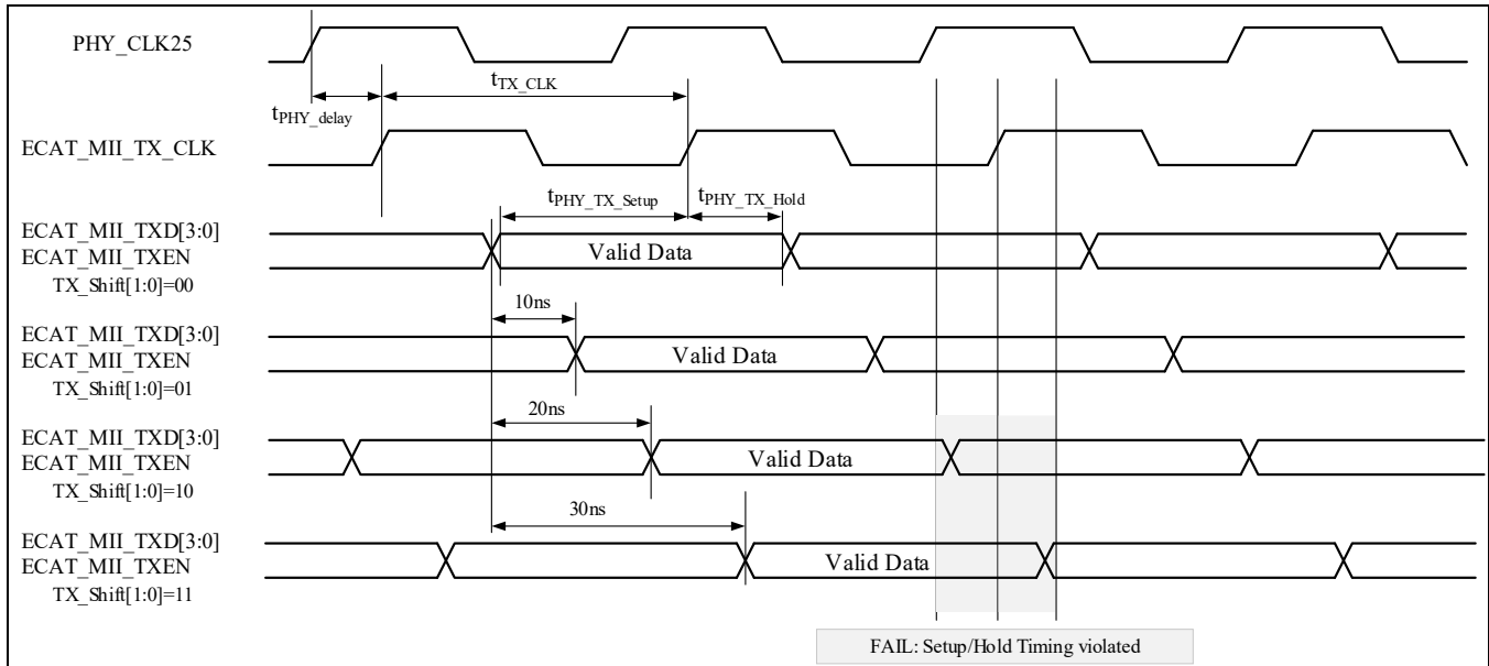
Figure 4-42 ESC MII TX Signal Timing Diagram
