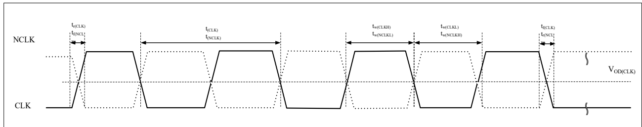
Figure 4-23 xSPI Hyperbus Clock Read Timing Diagram
