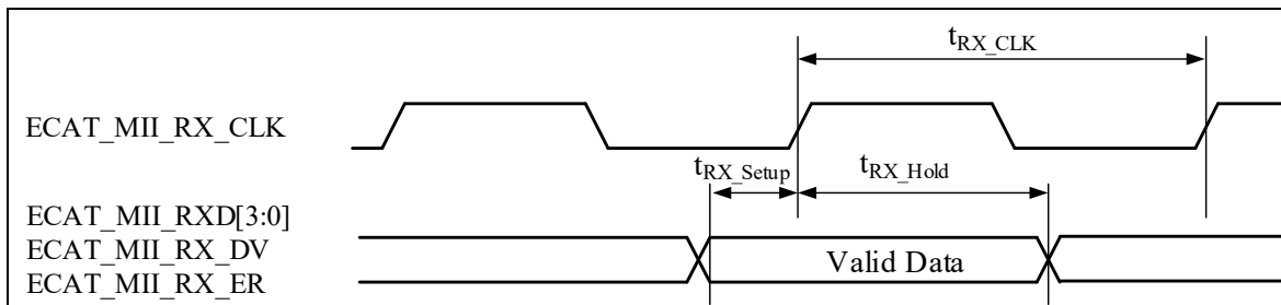
Figure 4-43 ESC MII RX Signal Timing Diagram
