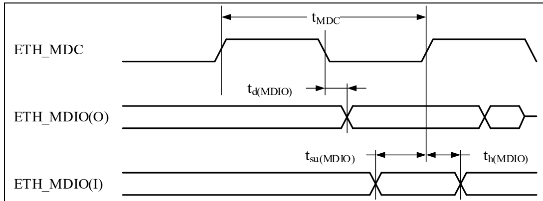
Figure 4-38 MDIO/SMA Timing Diagram
