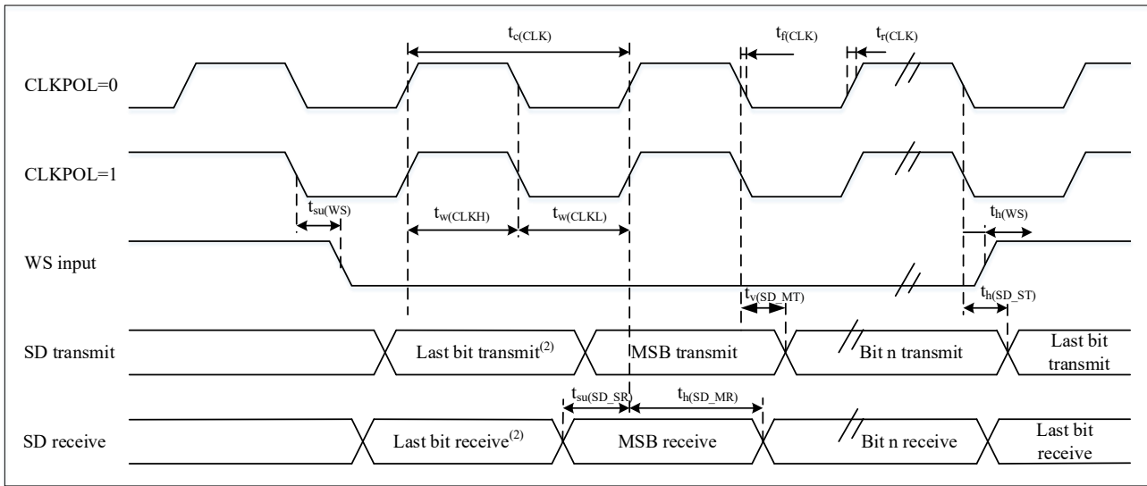
Figure 4-18 I2S Slave Mode Timing Diagram (Philips Protocol) (1)
