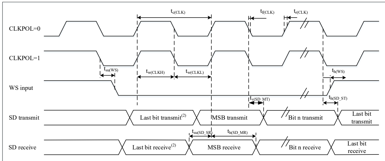
Figure 4-19 I2S Master Mode Timing Diagram (Philips Protocol) (1)
