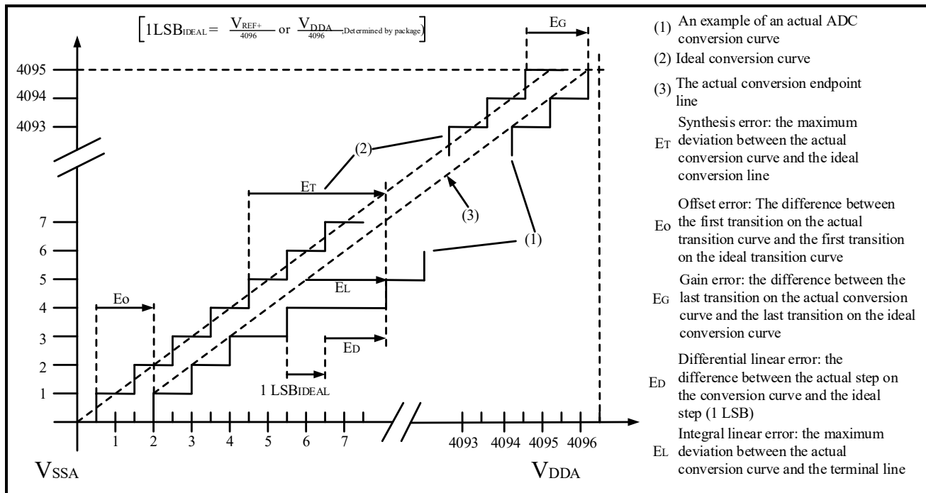
Figure 4-45 ADC Accuracy Characteristics
