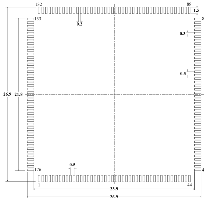
Figure 5-4 Design Recommendations for LQFP176 Package Pads (1)
