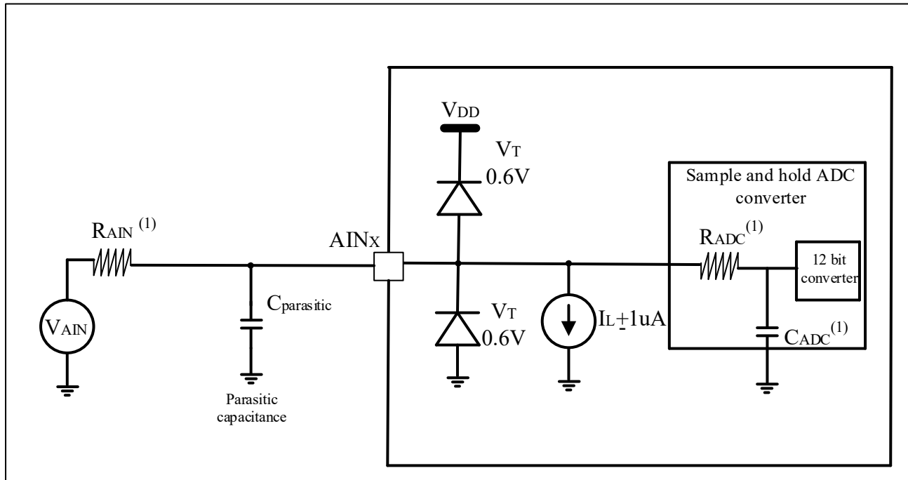
Figure 4-46 Typical Connection Diagram Using ADC
