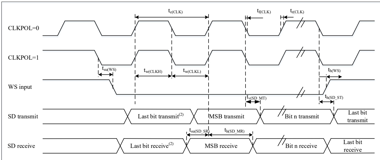
Figure 4-18 I2S Slave Mode Timing Diagram (Philips Protocol) (1)
