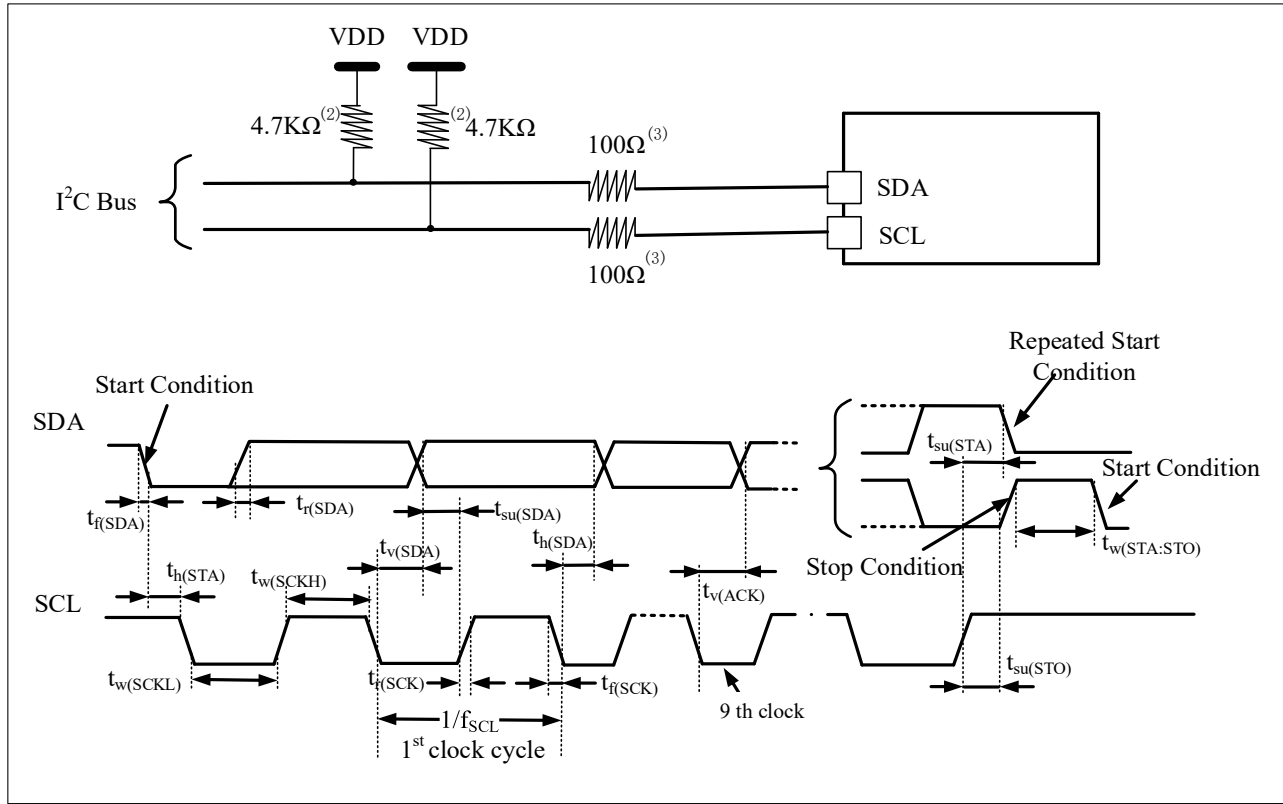
Figure 4-14 I 2 C Bus AC Waveform and Measurement Circuit (1)
