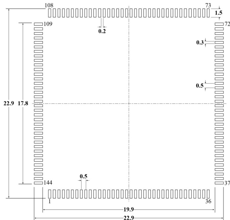
Figure 5-2 Design Recommendations for LQFP144 Package Pads (1)
