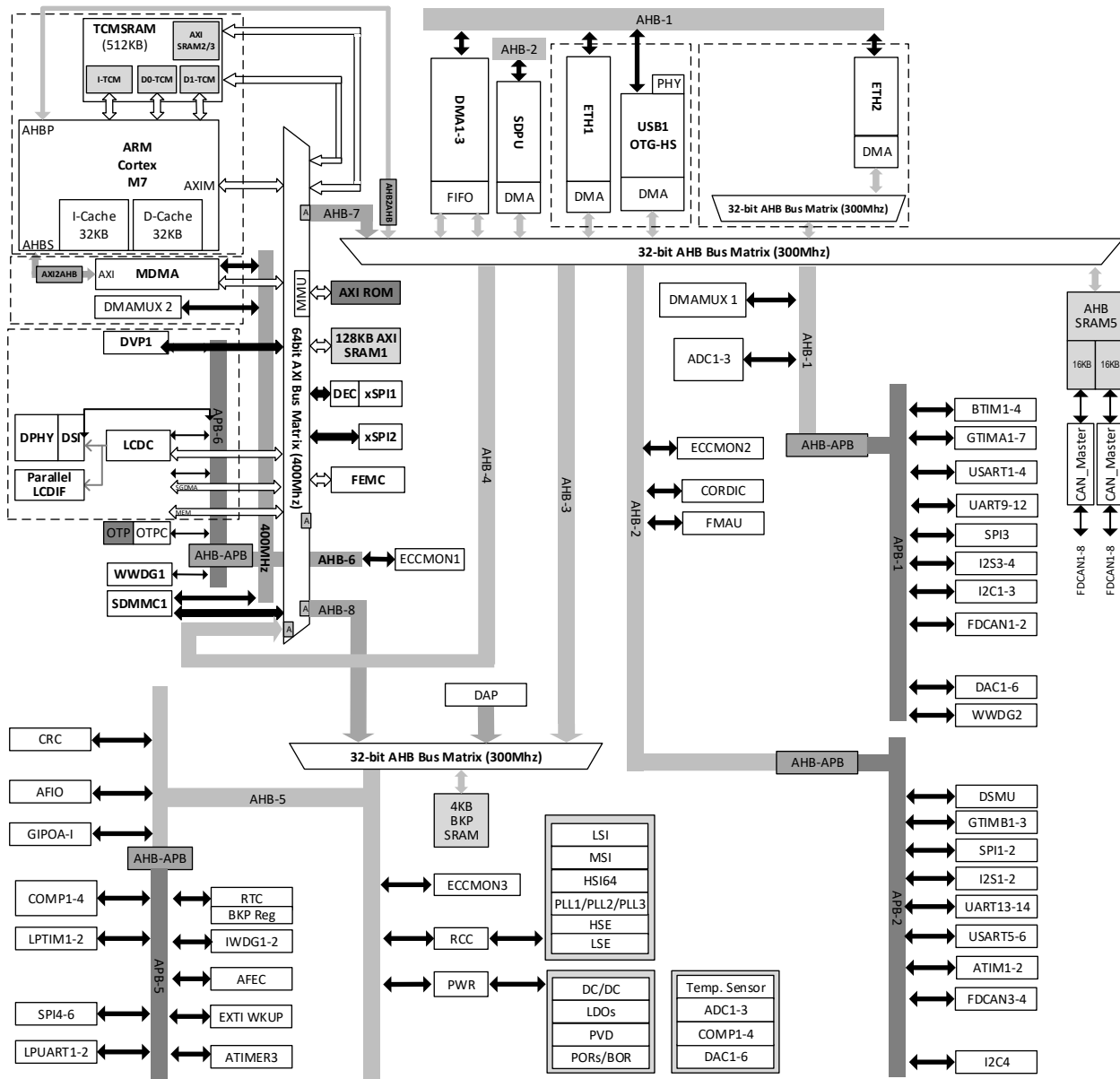
Figure 1-1 N32H735 System Block Diagram
