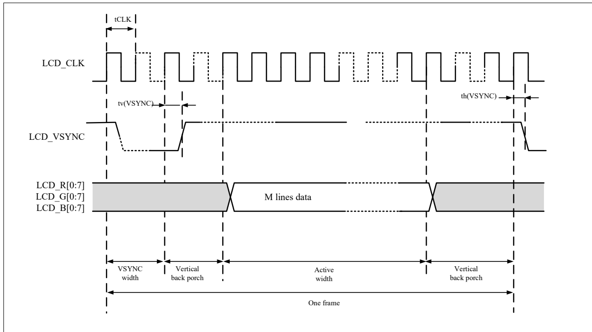
Figure 4-43 LCD-TFT vertical timing diagram
