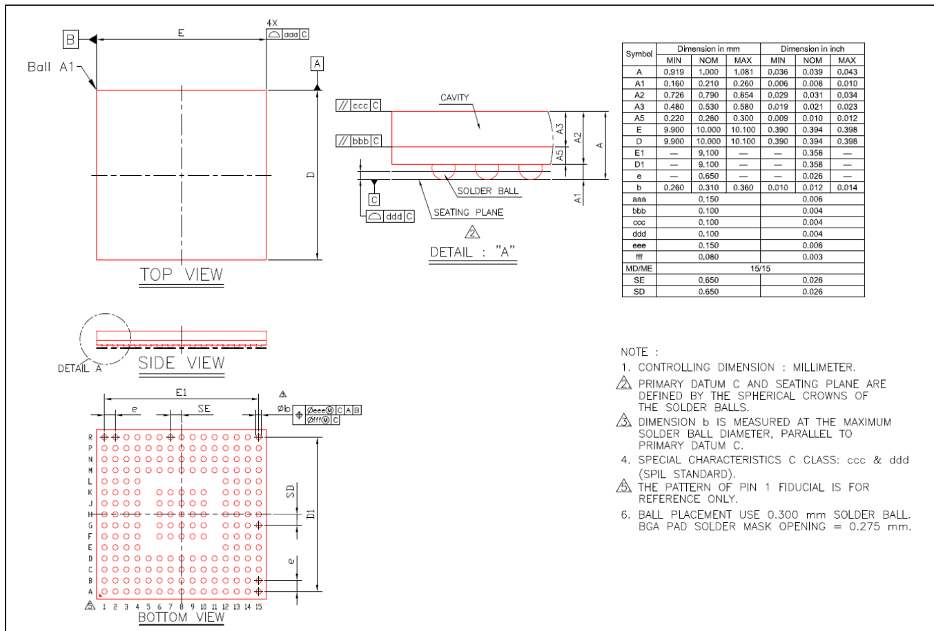
Figure 5-5 BGA176+25 Package Dimension
