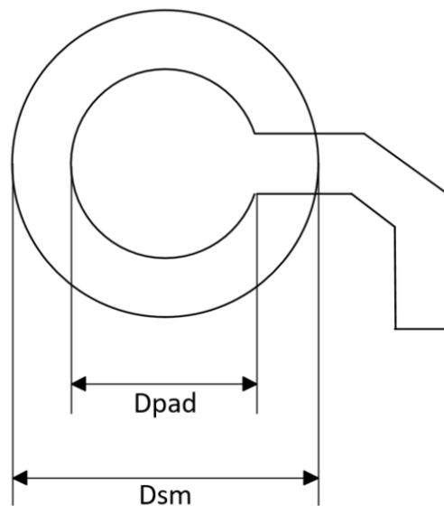
Figure 5-6 Recommended Pads for BGA176+25 Package
