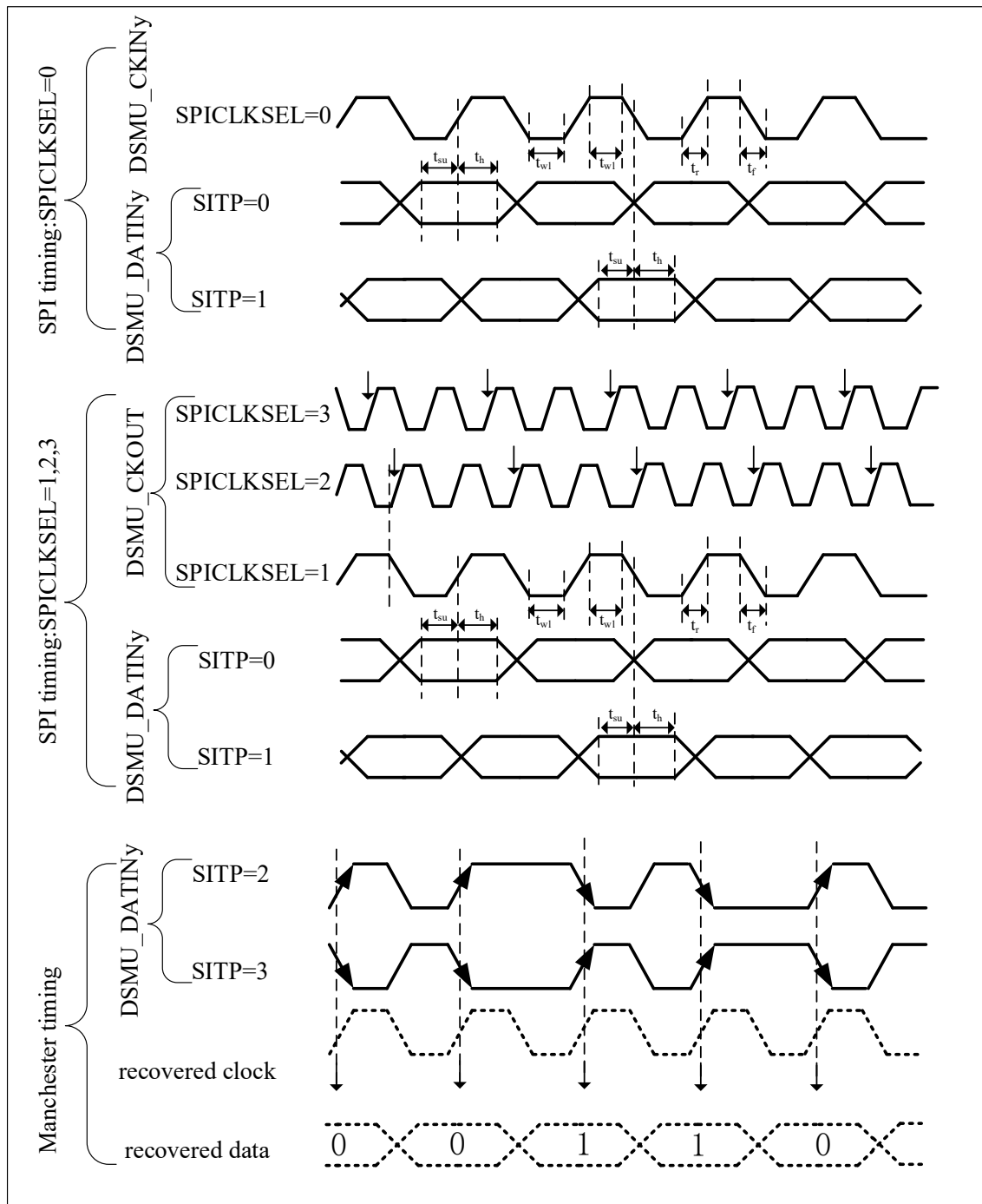
Figure 4-44 DSMU Channel Transceiver Timing Diagram
